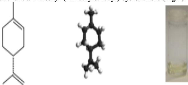
General structure Ball and stick Model Liquid form of limonene
