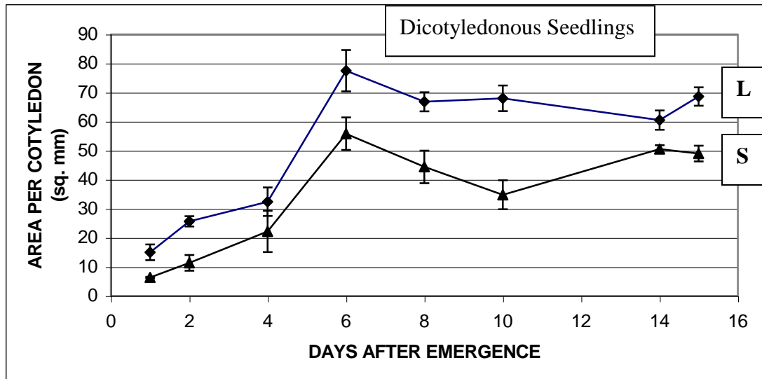
Fig. 5. Area of large (L) and small (S) cotyledons as a function of time in dicotyledonous seedlings of Opuntia .
