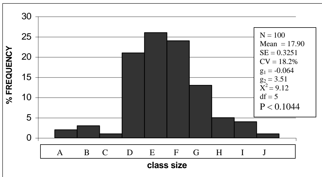
Fig. 1. Seed weight (mg / seed) distribution of Opuntia ficus-indica . Class sizes: A, 8–10 mg; B, 10.1–12 mg; C, 12.1–14, mg .....J, 26.1 to 28 mg per seed. The hypothesis that population is normal of mean 17.90 and SD 3.2513 cannot be rejected at the 95% confidence level.
