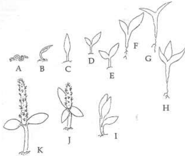
Fig.4. Various aged seedlings of Opuntia ficus-indica . A: hypocotyl emerging from soil; B: hypocotyl on emergence is bent hood of snake and generally bears two unequal cotyledons; C: hypocotyl takes around few hours to become erect while cotyledons still closely pressed; D & E: cotyledons open on second day of emergence; F & G: fifteen day old seedlings as seen from different angles; H: fifteen day old tricotyledonous seedlings; I: A 15 day old tricotyledonous seedling bearing a cotyledon abnormally – inserted nearly midway on the hypocotyls; J & K: nearly 2.5 months old dicotyledonous and tricotyledonous seedlings bearing phylloclade.
