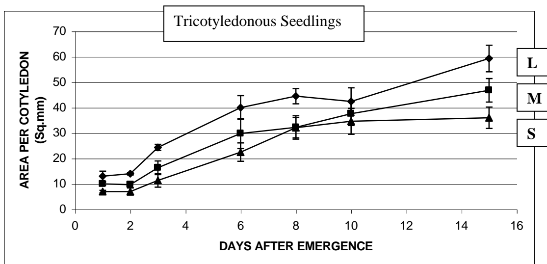
Fig.6. Area of large (L), medium (M) and small (S) cotyledons of tricotyledonous seedlings of Opuntia as a function of time.
