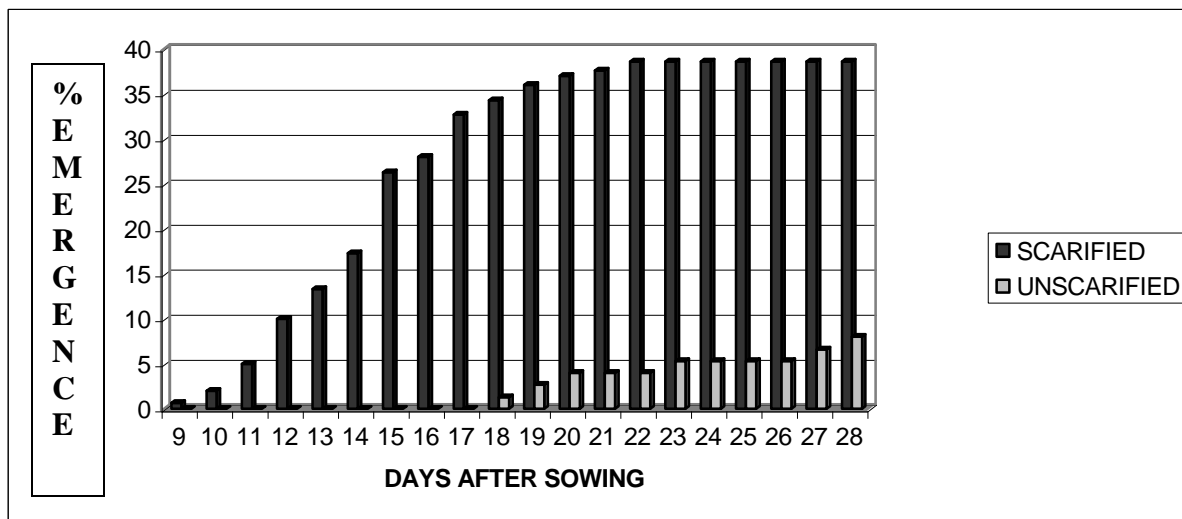
Fig. 2. Seedling Emergence from unscarified and chemically scarified (Conc. H 2 SO 4 for 2 minutes) seeds of Opuntia ficus-indica .
